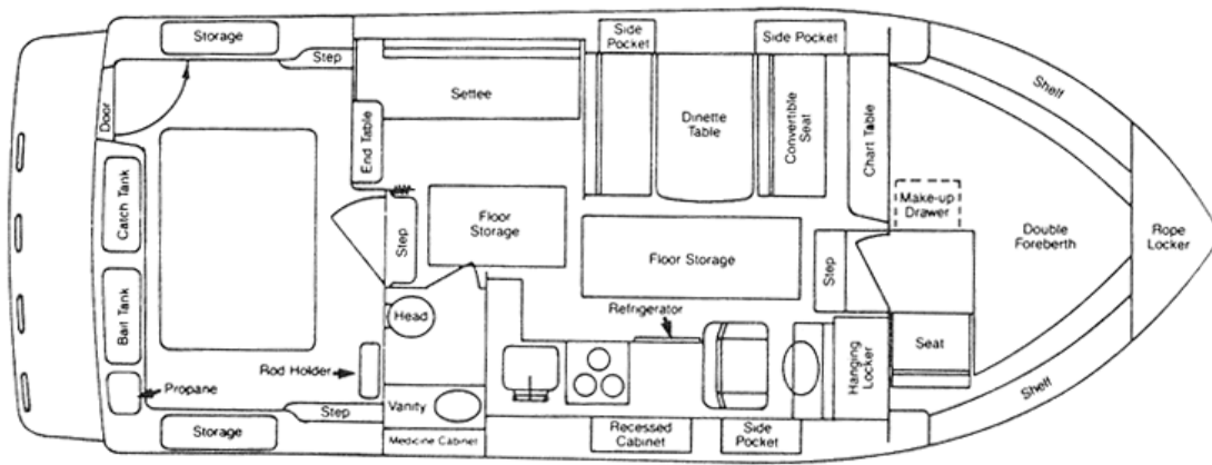
30' STANDARD PLAN
