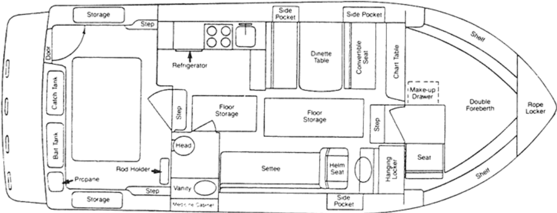
30' ALTERNATE PLAN
